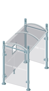
Length 2500 mm with two side claddings
